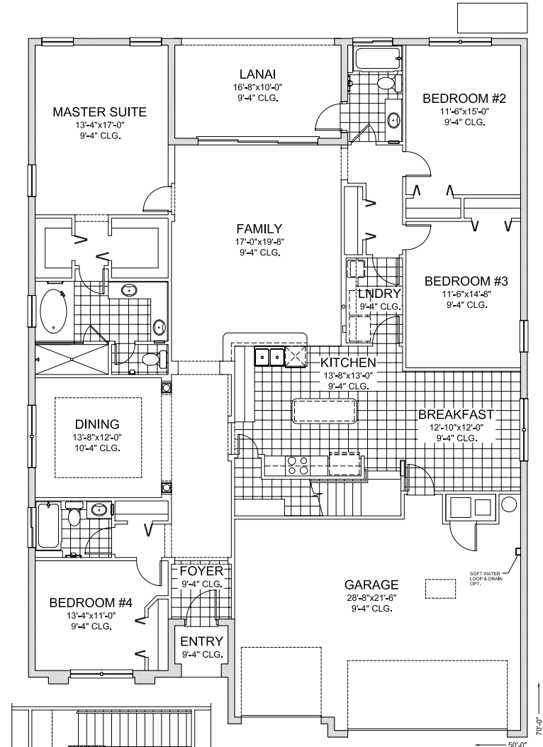
Floor Plan
